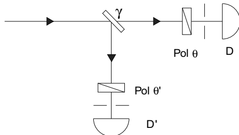
Figure 3: Which-way polarization measurement of a photon.
