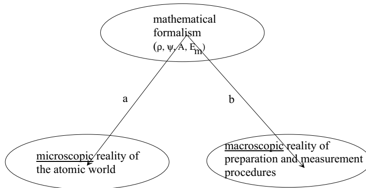
Figure 1: Realist (a) and empiricist (b) interpretations of the mathematical formalism of quantum mechanics.
