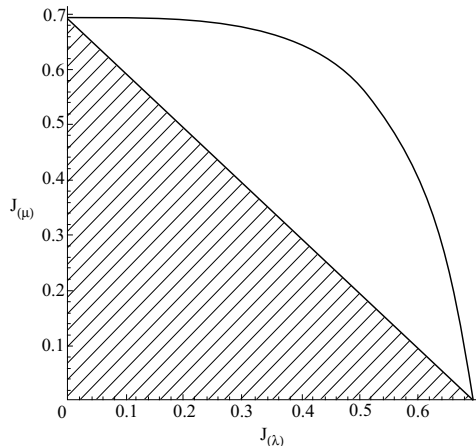
Figure 4: Parametric plot of J(\lambda) versus J(\mu) as a function of \gamma .
