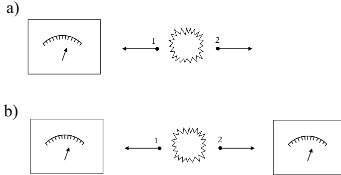
Figure 2: a) EPR experiment ; b) EPR-Bell experiment .
